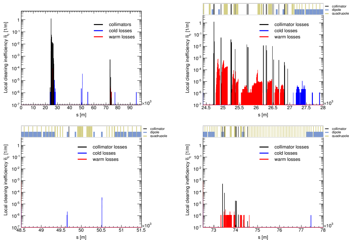
Fig. 5: Horizontal loss map at injection energy of 3.3 TeV for the entire ring (top left), zoom in the betatron cleaning insertion ESS-D (top right), in the interaction point G (bottom left) and in the momentum cleaning insertion ESS-J (bottom right) [23]. The interaction points A and G are located at s = 0 and 50 \times 10^3 m respectively, while ESS-D and ESS-J start at about s = 23 \times 10^3 and 73 \times 10^3 m respectively.
