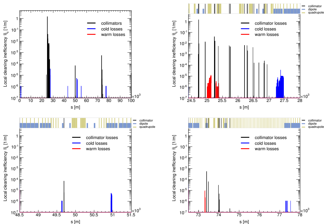
Fig. 6: Horizontal loss map at collision energy of 50 TeV for the entire ring (top left), zoom in the betatron cleaning insertion ESS-D (top right), in the interaction point G (bottom left) and in the momentum cleaning insertion ESS-J (bottom right) [23]. The interaction points A and G are located at s = 0 and 50 \times 10^3 m respectively, while ESS-D and ESS-J start at about s = 23 \times 10^3 and 73 \times 10^3 m respectively.
